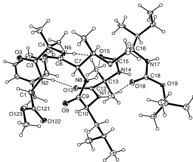
Figure 3. The ORTEP diagram of peptide II including atom numbering scheme. Thermal ellipsoids are shown at the level of 25% probability. Hydrogen bonds are shown as dotted lines.
