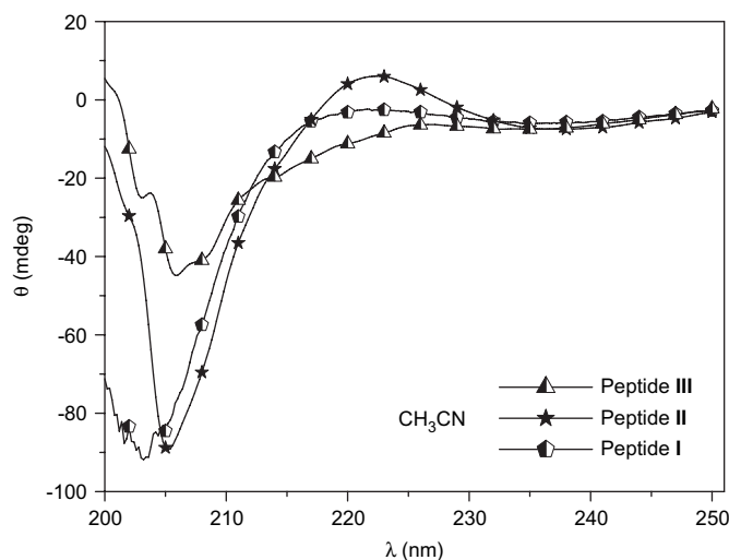
Figure 8. CD curves of peptides I – III in acetonitrile (1.5 mM).
