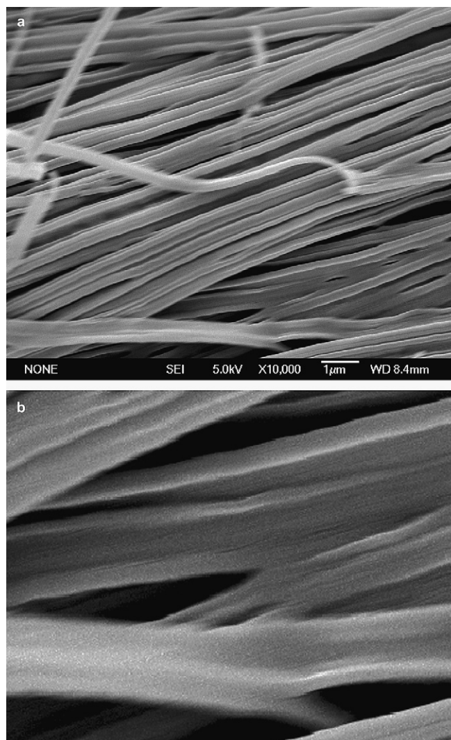
Figure 9. (a) FE-SEM image ( \times 10,000 ) of peptide II showing the formation of non-twisted ribbon-like structures. (b) The enlarged SEM image clearly demonstrates that the ribbons are formed through lateral association of non-twisted filaments.
