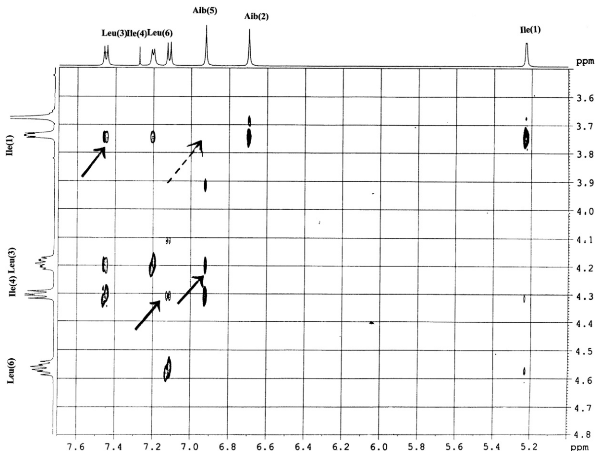
Figure 7. Section of the ROESY spectrum of peptide I in \text{CDCl}_3 (peptide concn: 1 \times 10^{-2} M). The [d_{\alpha\text{N}}(i, i+2)] , where i=1, 3 , and 4 crosspeaks typical of a 3_{10} -helix are indicated (full arrow). The area in the spectrum where the undetected [d_{\alpha\text{N}}(i, i+4)] , where i=1 crosspeak typical of an \alpha -helix was expected is also marked (dashed arrow).
