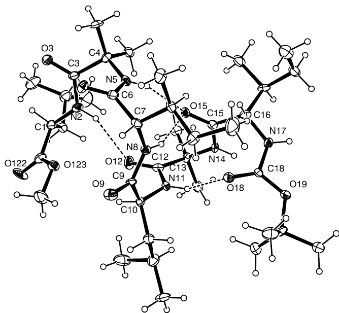
Figure 2. The ORTEP diagram of peptide I including atom numbering scheme. Thermal ellipsoids are shown at the level of 25% probability. Hydrogen bonds are shown as dotted lines.
