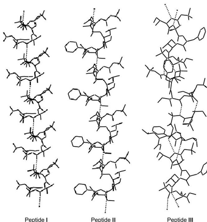
Figure 5. Packing diagrams of peptides I–III showing the formation of supra-molecular helices. Intermolecular hydrogen bonds are indicated by dotted lines. Peptides I and II show one hydrogen bond between molecules related by translational symmetry along the a axis while peptide III shows two hydrogen bonds between adjacent molecules around the 3_1 screw axis.
