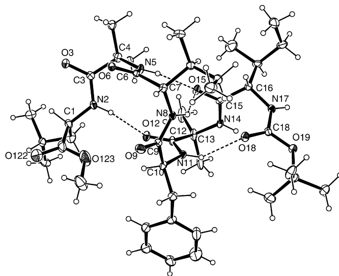
Figure 4. The ORTEP diagram of peptide III including atom numbering scheme. Thermal ellipsoids are shown at the level of 25% probability. Hydrogen bonds are shown as dotted lines.
